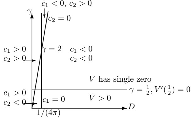
FIGURE 2. Regions of in/stability of first and second eigenvalue
