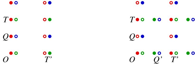
FIGURE 4. The possible arrangements of the divisors of x_1 \circ \psi_1 (red), x_2 \circ \psi_2 (green) and x_3 \circ \psi_3 (blue). On the left is Scenario (1), on the right Scenario (2). • denotes a zero, ◦ a pole of x_j \circ \psi_j .
